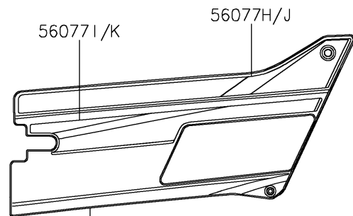
Ref.Door
