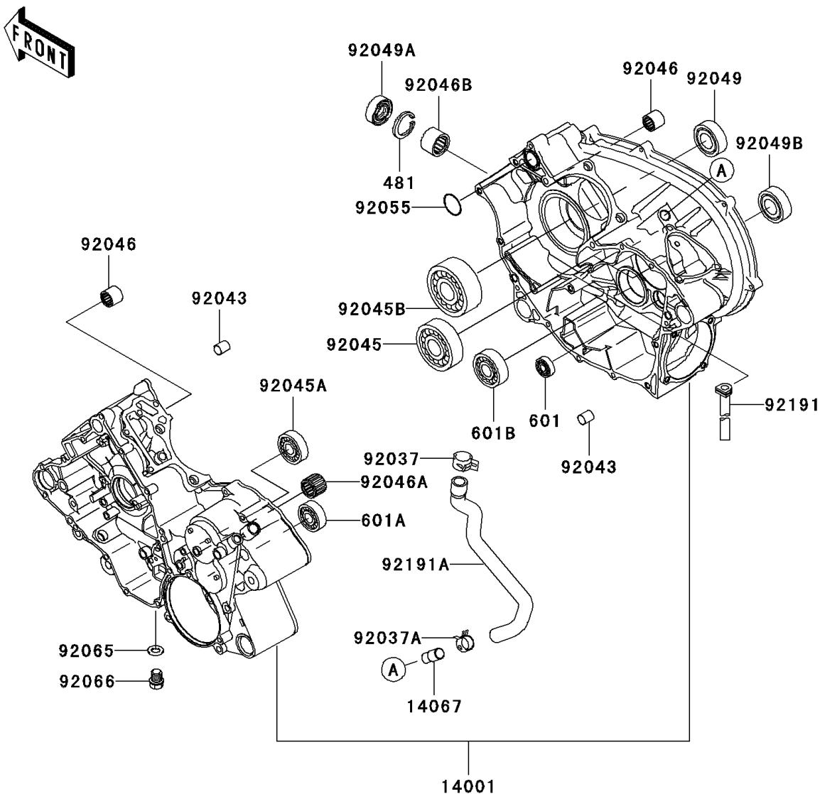
(14001 LH Side)
