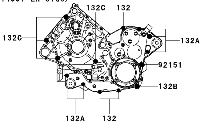
(14001 LH Side)
