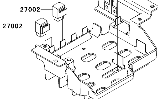
Ref. Frame Fittings (Rear)
